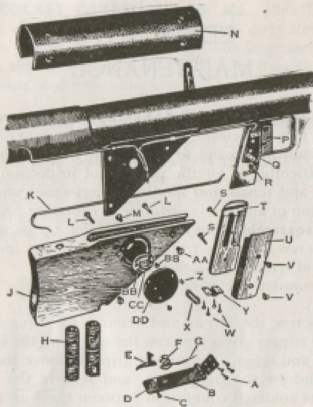
Figure 35. Stock and grip group, launcher M1A1.
