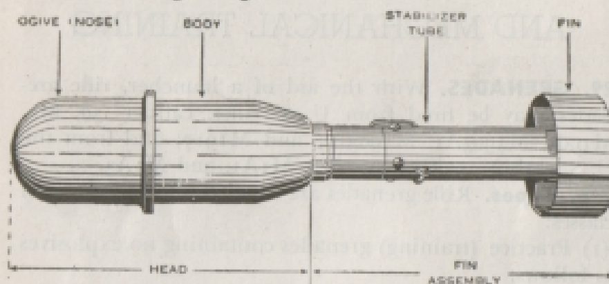
Figure 14. Nomenclature of antitank rifle grenades.
