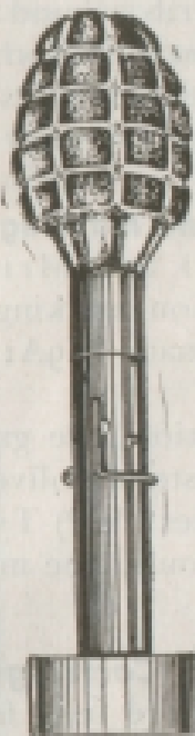
Figure 17. Impact fragmentation rifle grenade M17 (formerly the T2).
