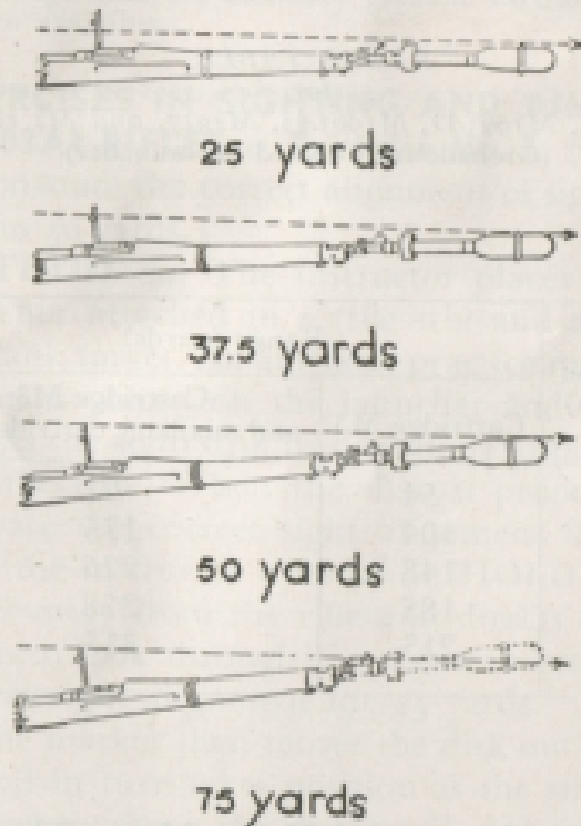
Figure 27. Method of aiming grenades M9A1, M11A1, and M11A2, with M1903 and M1903A1 rifles.
