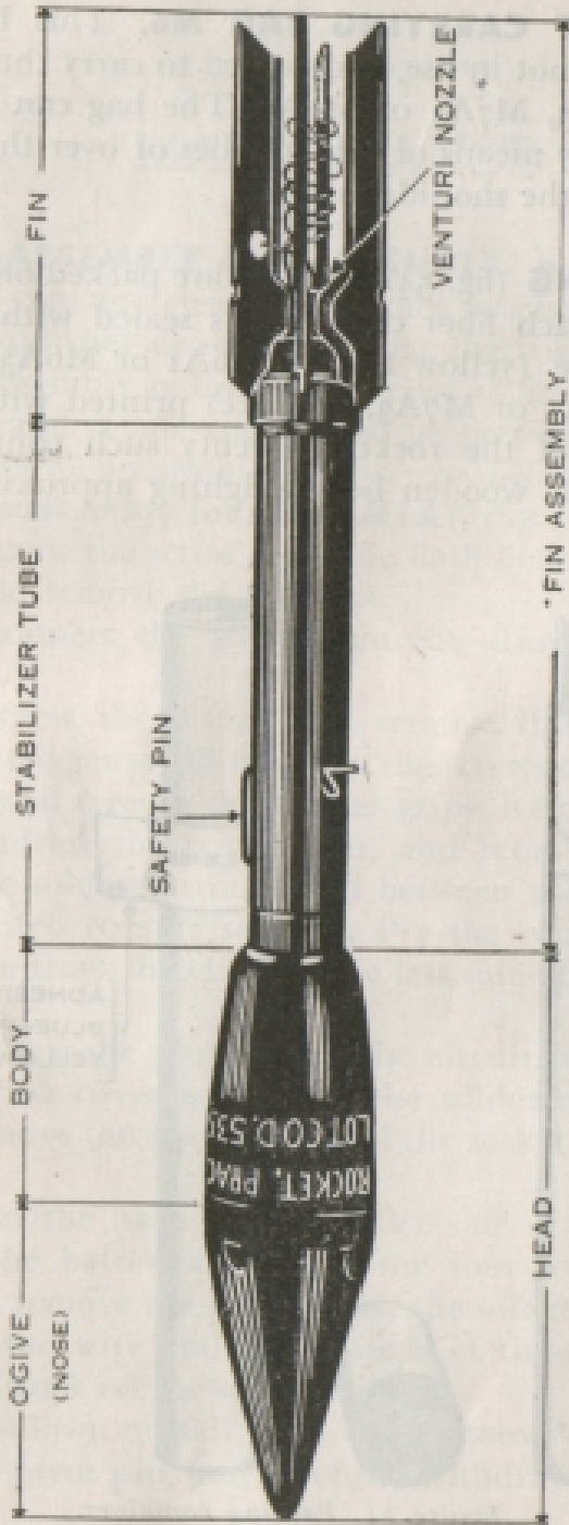
Figure 53. Practice antitank rocket, 2.36-inch, M7Ar.
