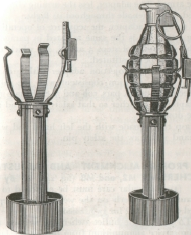
⊙ Grenade projection adapter M1, with hand grenade Mk. II.
