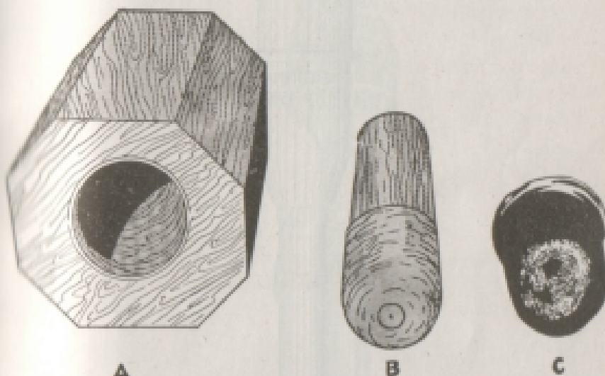
① Punch and die used for straightening dented nose (ogive). A - Die, B - Punch, and C - Dented nose.
