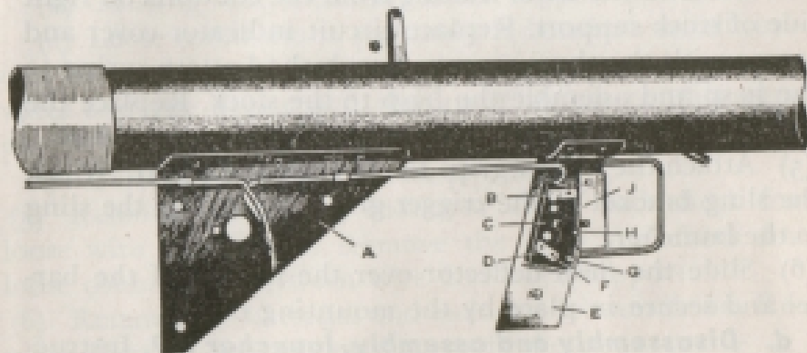
Figure 56. Trigger group, launcher M1A1.
