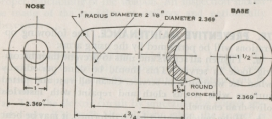
② Large dent remover, 2.369 inch diameter.
